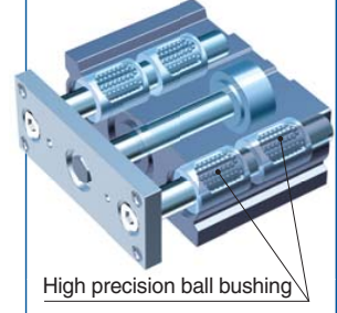
Ball bushing
