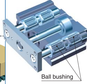
High precision ball bushing
