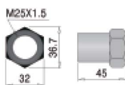
RSC25-1-XLC01
