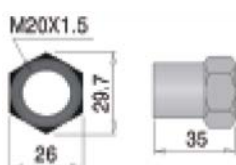
RSC20-XLC01
