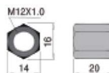
RSC12-XLC01
