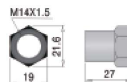
RSC14-XLC01
