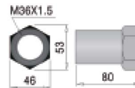
RSC36-XLC01
